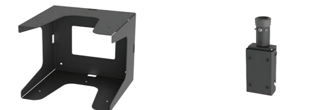
Example wall mount for Martin Audio SX-112.
